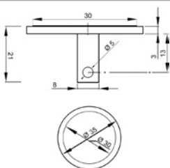
Easy-Glue, Easy-Steel, Easy-Ring, glasbord
